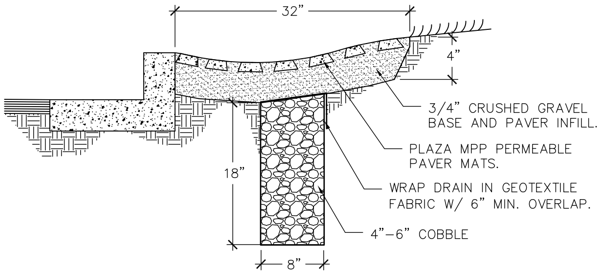
PERMEABLE PAVER EDGE WITH GRAVEL DRAIN
